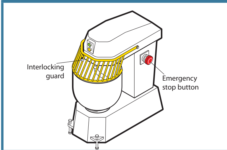
FIGURE 2: Food mixer with interlocking arm
