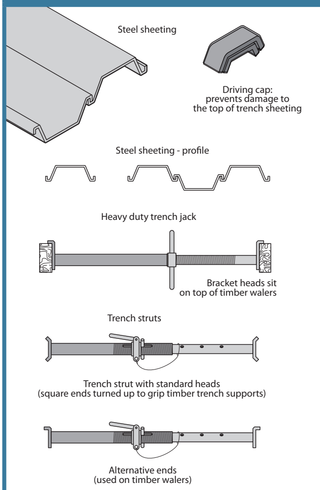
FIGURE 14 Steel trench sheeting and jacks
