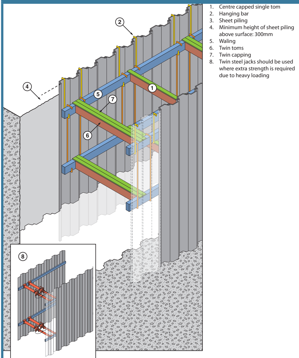
FIGURE 13 Steel sheet piling
