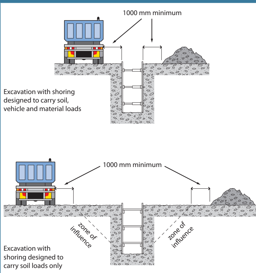
FIGURE 2 Excavated material and loads near excavations
