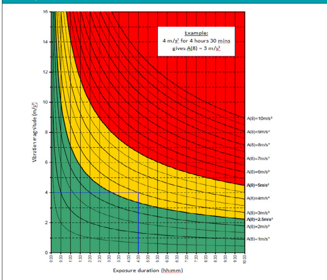
Figure 2 Graph for determining daily vibration exposure A(8) from vibration magnitude and exposure duration
