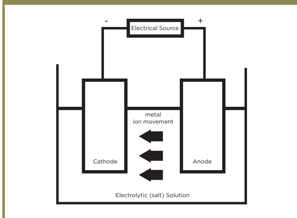
FIGURE 1: Electroplating system
