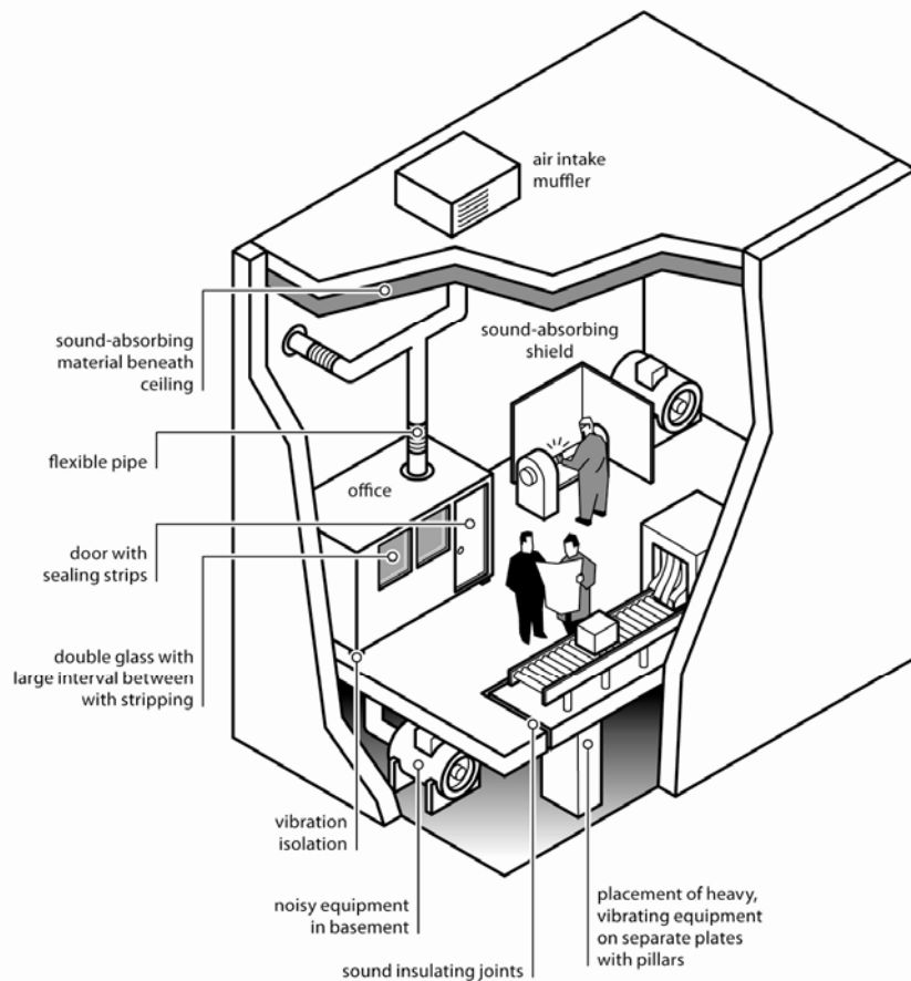
Figure 3: Examples of noise control measures in an industrial building
